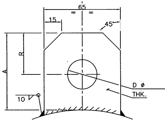
LIFTING LUG FOR SHELL COVER, CHANNEL AND CHANNEL COVER
