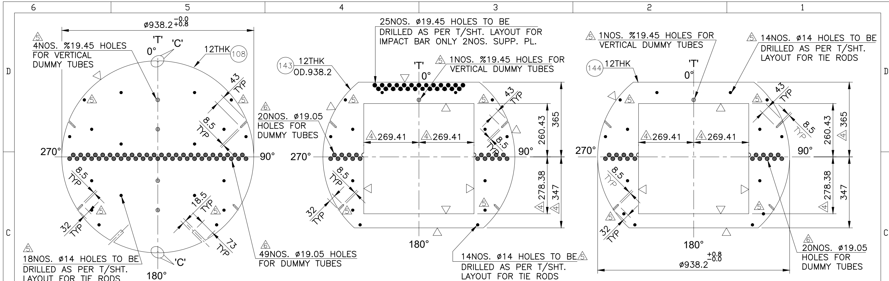
DETAIL OF ADDITIONAL PARTIAL SUPPORT PLATE 'S1'
